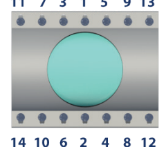
FIGURE 7 10" and 12" Bolt Tightening Pattern
